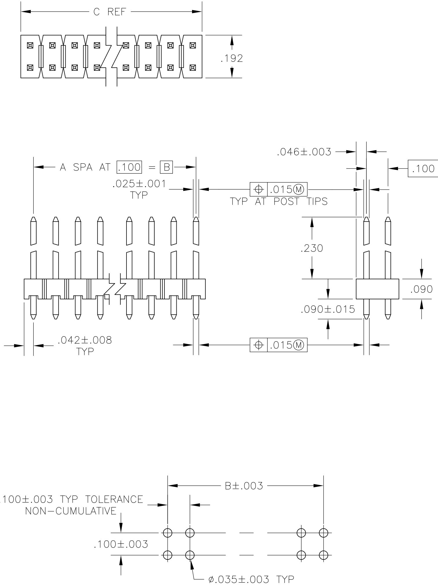
RECOMMENDED HOLE LAYOUT
